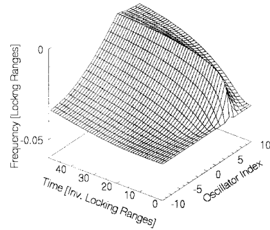
Fig. 6. Frequencies of the oscillators of Fig. 8.
