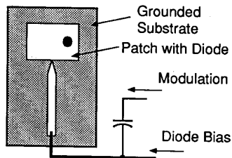
Fig. 2. Active radiating element, using a patch antenna and Gunn diode. Bias is applied at an RF null on the patch, and modulation signals are capacitively coupled to the bias line.
