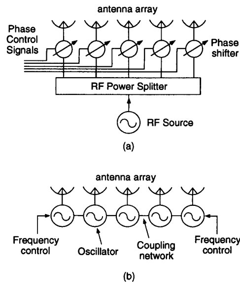
Fig. 1. (a) Block diagram of a conventional phased-array system for beam-scanning, and (b) Illustration of the proposed technique. The dynamics of the injection-locking process establishes a constant phase progression across an array of coupled-oscillators when the end elements are detuned in a particular way.
