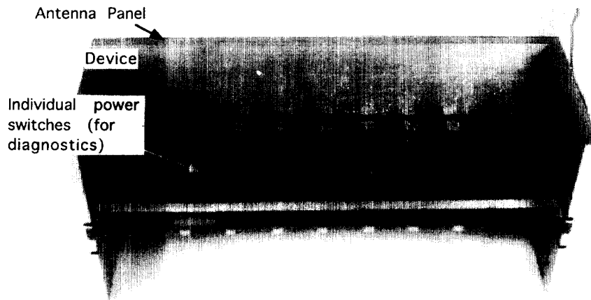
Figure 2b: Photograph of Oscillator Palette Antennas are fed thru holes drilled in ground plane of antenna palette.
