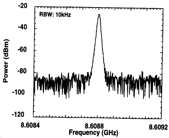
Fig.4 output spectrum of the array when low phase noise signal is injected
