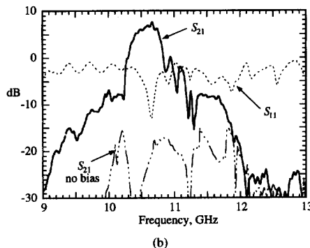
Fig. 3. (a) Picture of the amplifier cell with direct integration of 50- \Omega five-slot antennas and a commercial HBT gain block MMIC chip. The amplifier cell is fabricated on a 2.54 cm \times 2.54 cm Alumina substrate and the dimensions of the antennas are given in the paper. (b) The gain curve (direct measurement) of this amplifier cell in a square waveguide, with and without dc bias.
