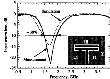
Fig. 1. The calculated and measured frequency response of a triple-slot antenna on 0.813-mm Duroid 5880 ( \epsilon_r = 2.2 ). The -10 -dB return loss bandwidth is approximately 30%.
