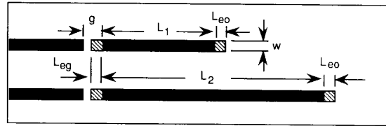
Fig. 1. Gap resonator pair for dispersion measurements. By measuring the resonant frequency of the two resonators end effects can be canceled.
