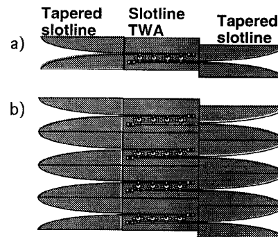
Figure 1 - Quasi-optical TWA a) single element b) Array
