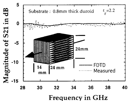
Figure 4- Ka-band results for a 16 x 19 passive array
